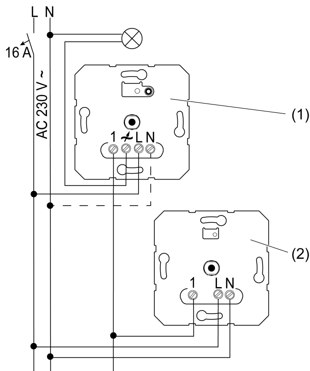
Figure 3: Connection example with rotary dimmer
