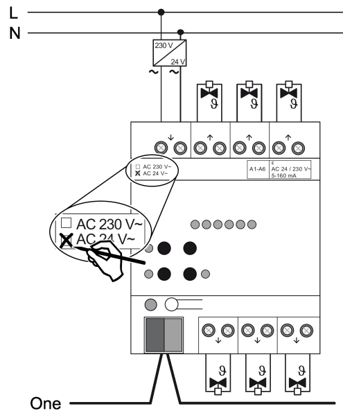
Image 4: Connection of 24 V valve drives
