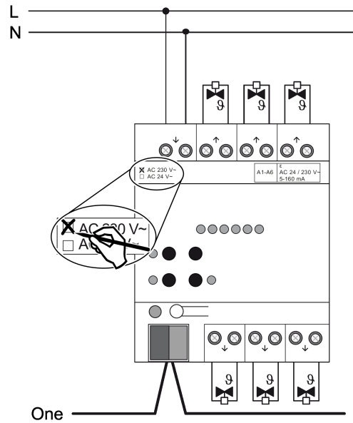
Image 3: Connection of 230 V valve drives
