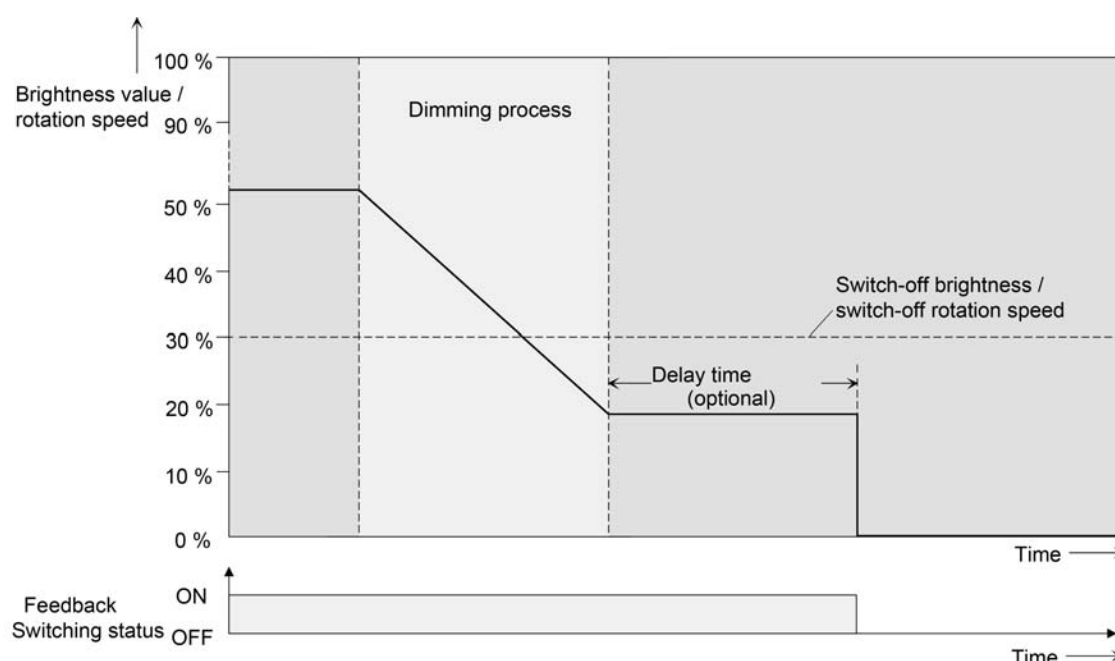
Figure 17: Dimming and switching behaviour of the automatic switch-off function
