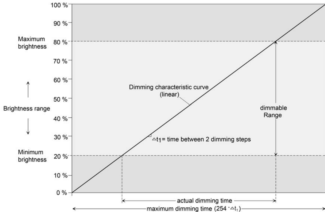
Figure 36: Linear characteristic dimming curve as an example with minimum brightness > 0 % and maximum brightness
