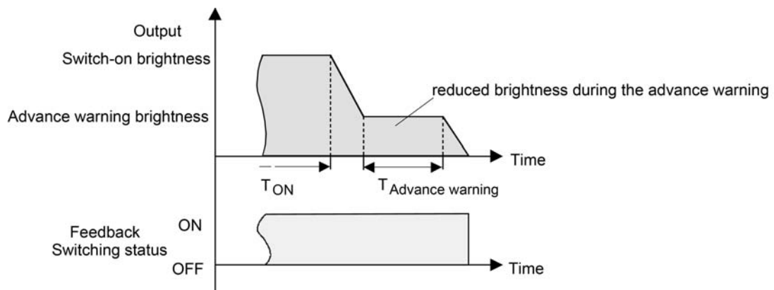
Figure 25: The pre-warning function of the staircase function with soft OFF function (for example with minimum brightness = 0 %)
