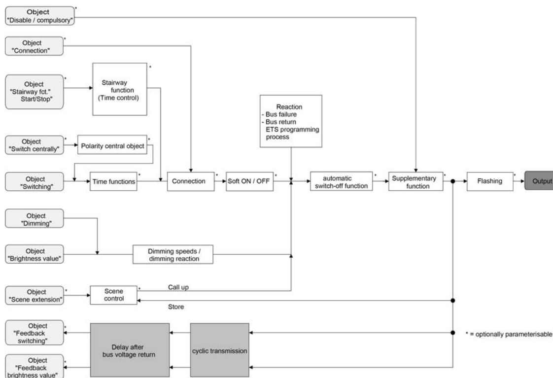
Figure 13: Functional feedback diagram of the feedbacks
